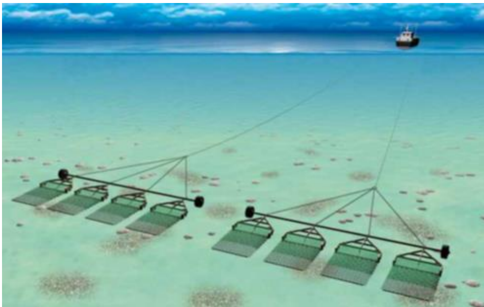
Figure 3.83.8 Typical dredge gear configuration (Source: Seafish, 2015)
