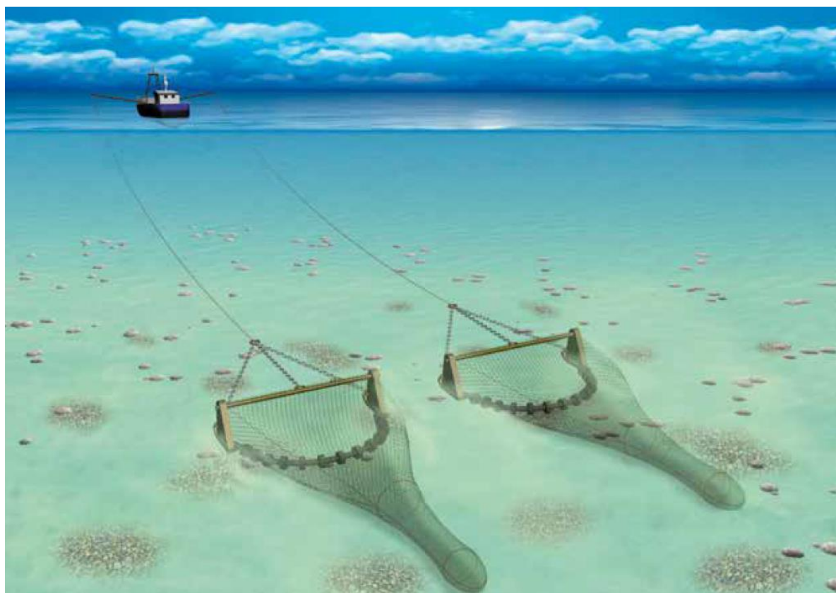
Figure 3.163-16 Typical beam trawl gear configuration (Source: Seafish, 2015)
